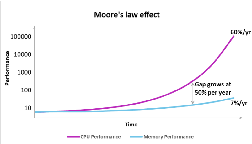
Figure 1 Historical performance gap between CPU and memory performance (Source: Synopsys)
