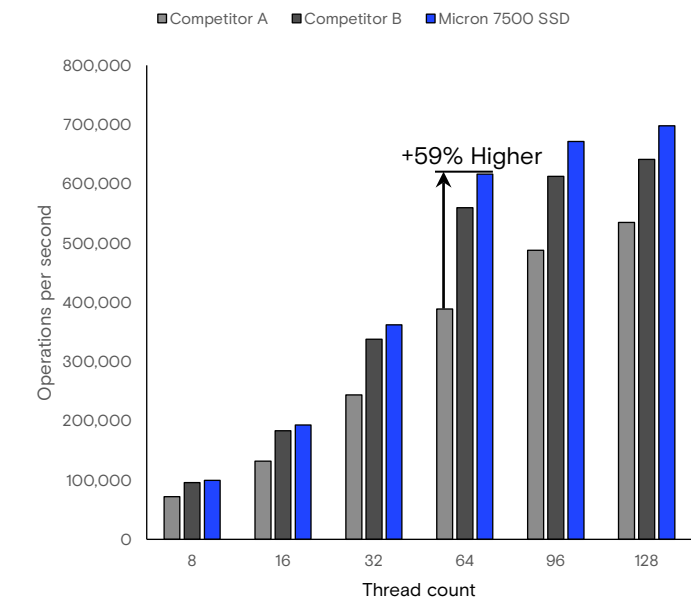
Figure 1: 4KB random read performance scaling by thread count
