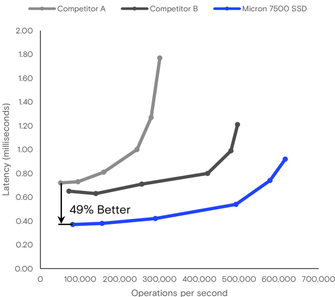
Figure 4: Application responsiveness vs. 4KB random read while writing performance
